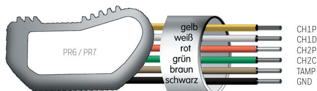
Pin assignment
